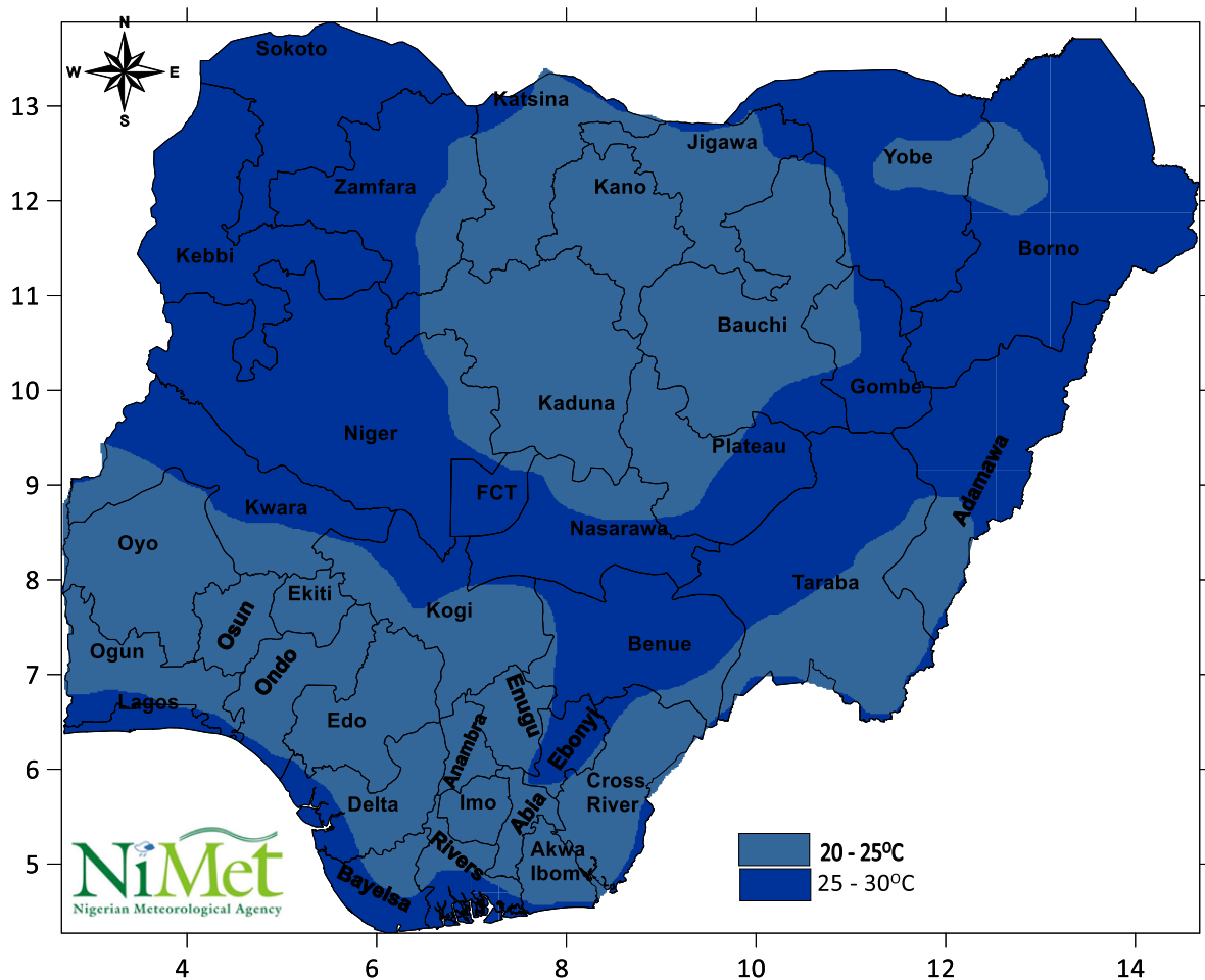
FIGURE 3: SPATIAL DISTRIBUTION OF MINIMUM TEMPERATURE FORECAST.
