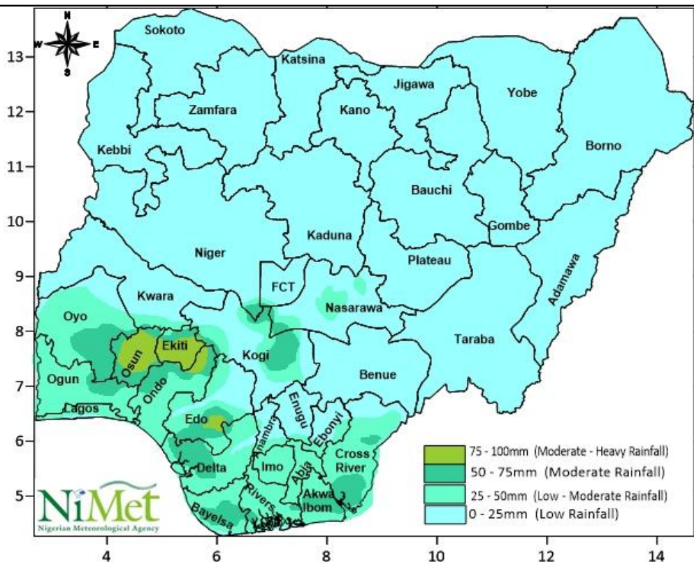
FIGURE 1: SPATIAL DISTRIBUTION OF ANTICIPATED RAINFALL.
